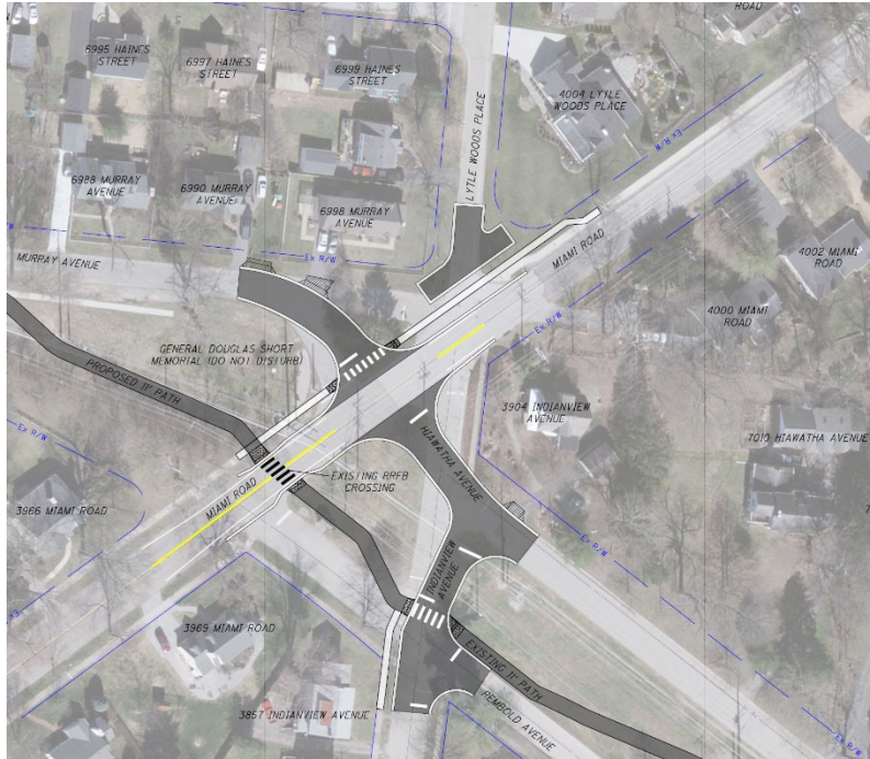
Figure 1: Potential Intersection Improvements
